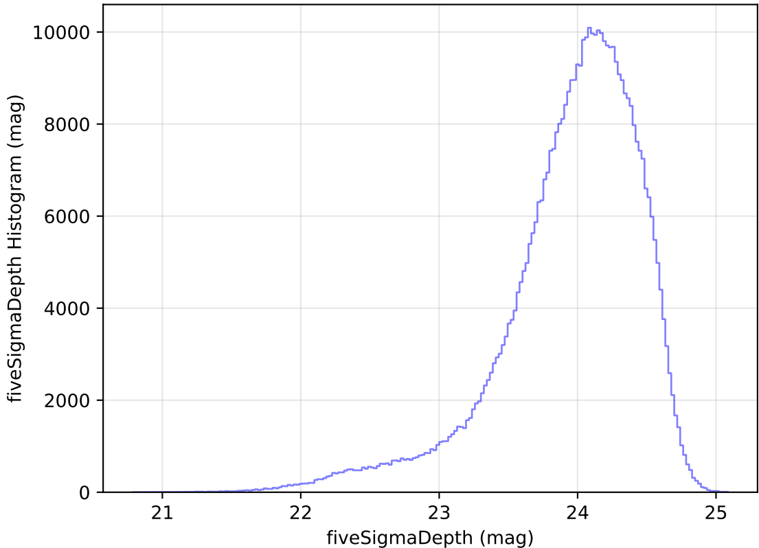
too_elab_r256_d3_ugrizy_v3.4_10yrs All sky r band: fiveSigmaDepth Histogram
