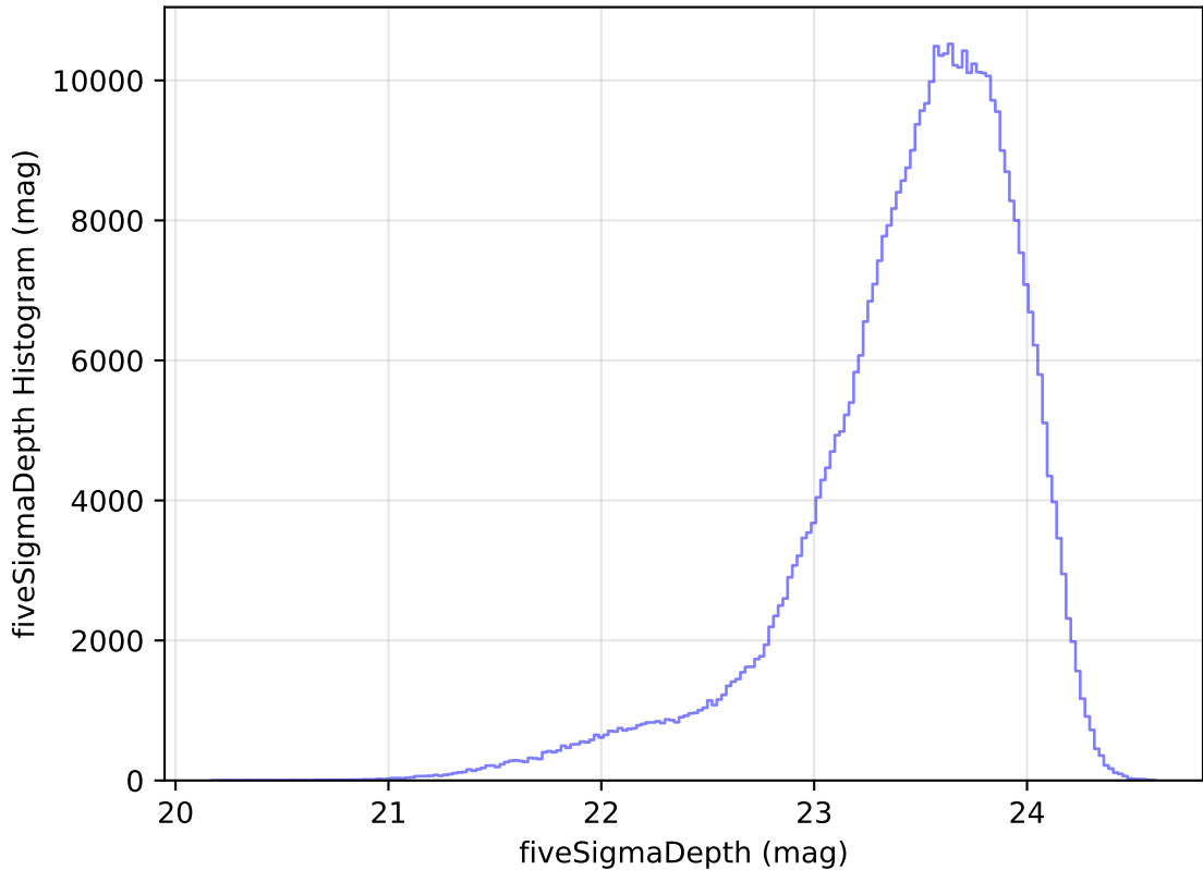
too_elab_r256_d3_ugrizy_v3.4_10yrs All sky i band: fiveSigmaDepth Histogram
