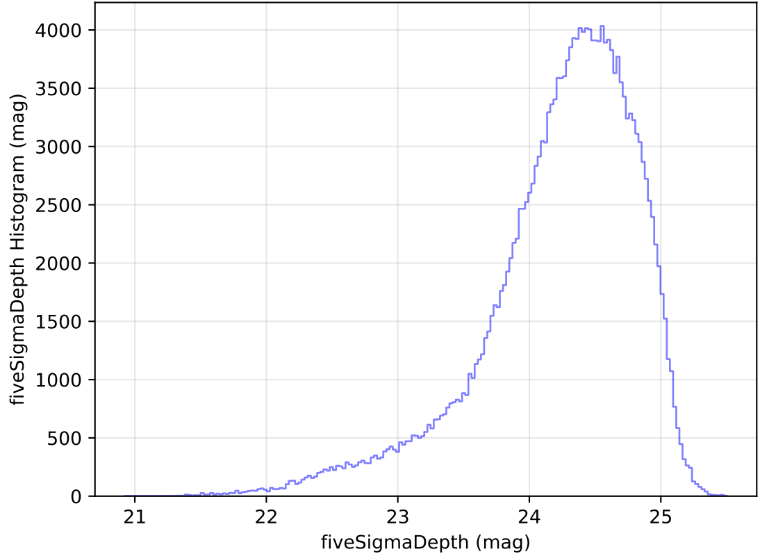
too_elab_r256_d3_ugrizy_v3.4_10yrs All sky g band: fiveSigmaDepth Histogram
