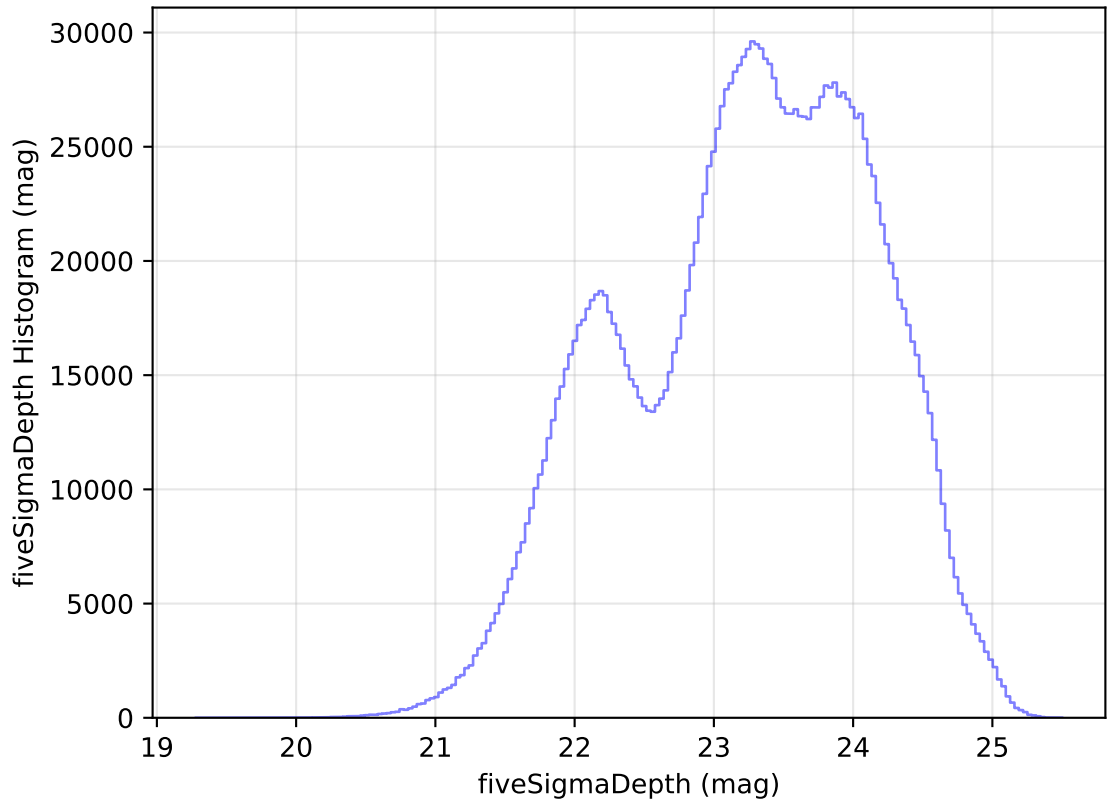
too_elab_r256_d3_ugrizy_v3.4_10yrs All sky all bands: fiveSigmaDepth Histogram
