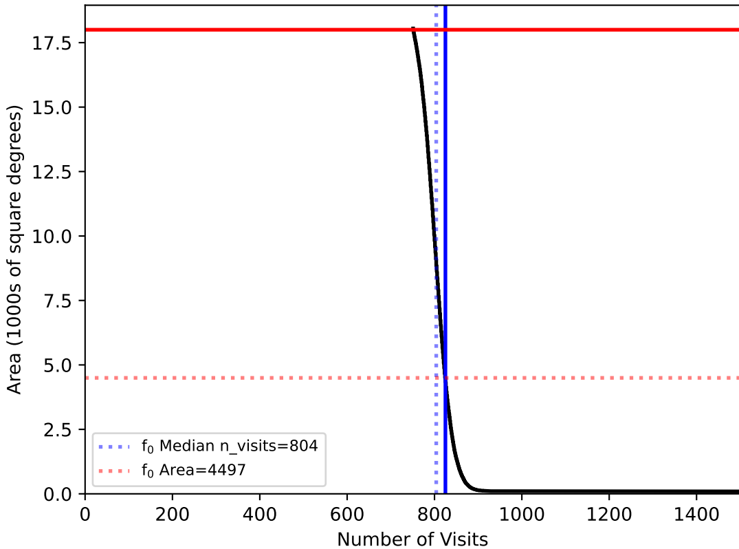
too_elab_r256_d3_ugrizy_v3.4_10yrs WFD: fO
