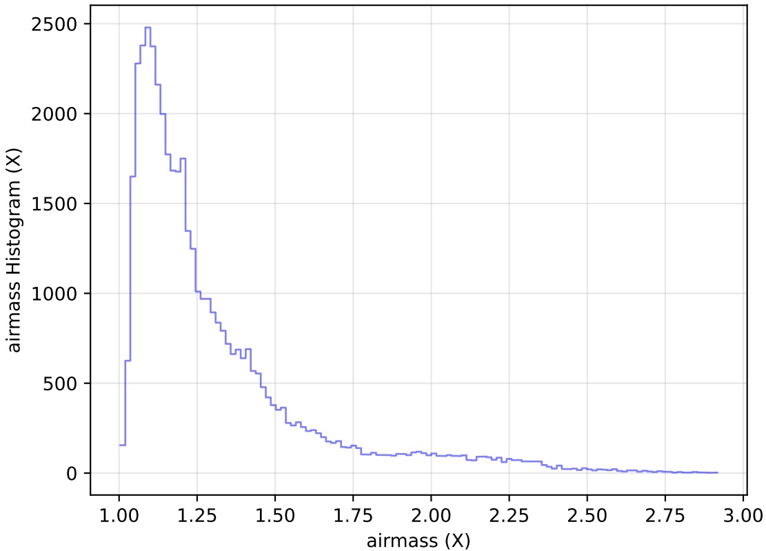
too_elab_r256_d3_ugrizy_v3.4_10yrs Yr 1 z band: airmass Histogram
