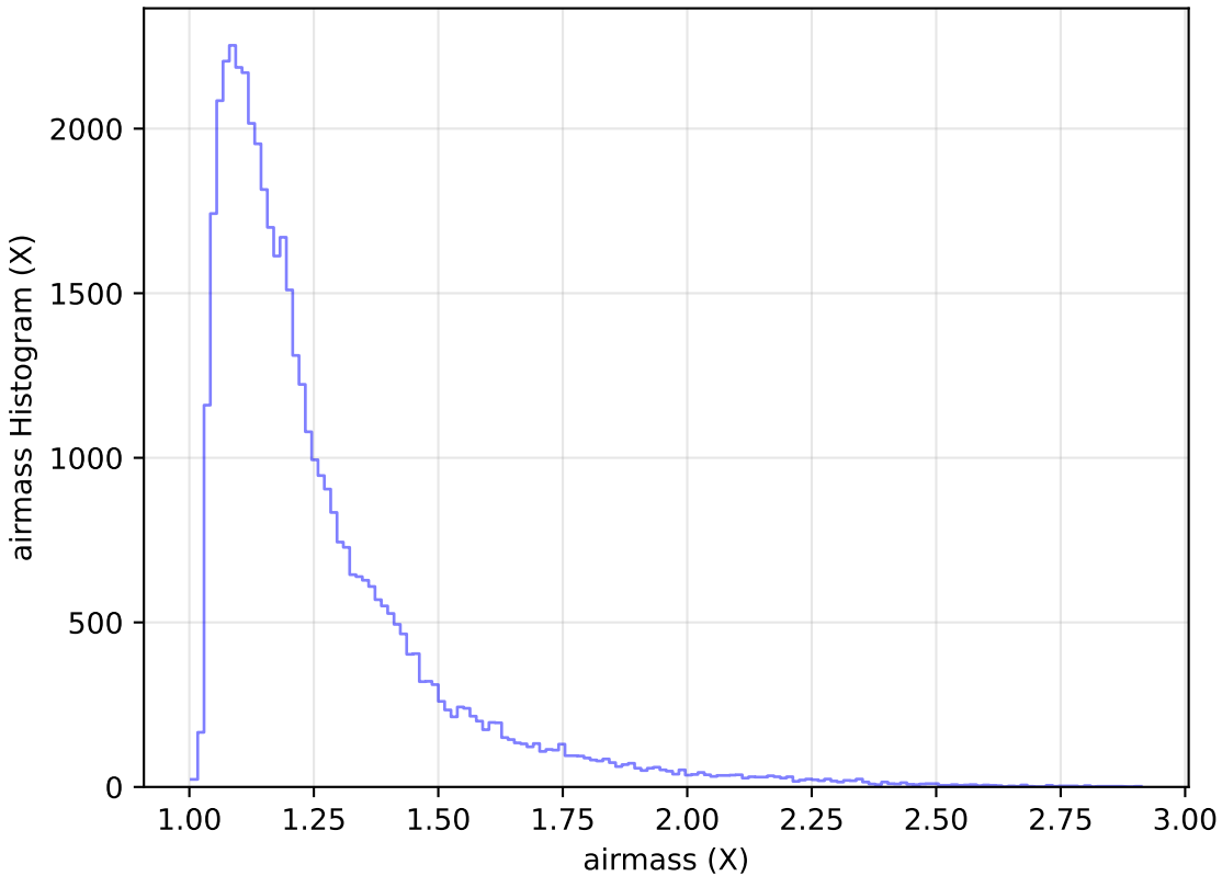
too_elab_r256_d3_ugrizy_v3.4_10yrs Yr 1 y band: airmass Histogram
