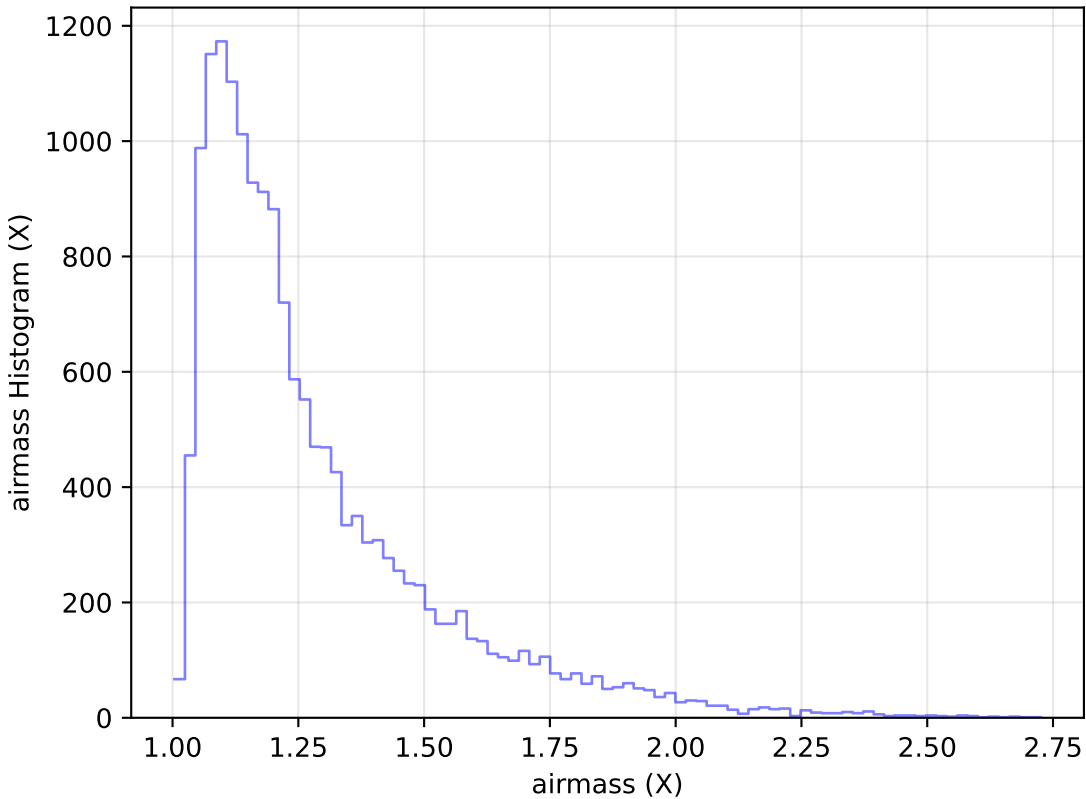
too_elab_r256_d3_ugrizy_v3.4_10yrs Yr 1 u band: airmass Histogram
