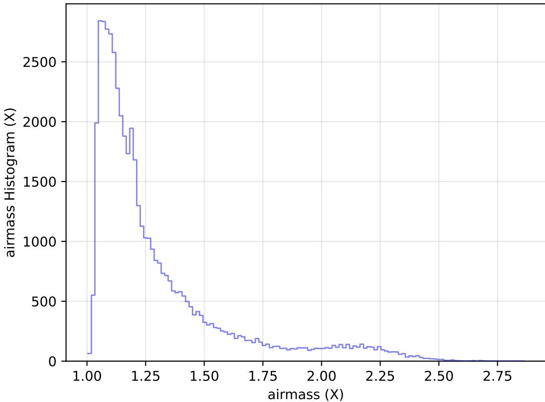
too_elab_r256_d3_ugrizy_v3.4_10yrs Yr 1 r band: airmass Histogram
