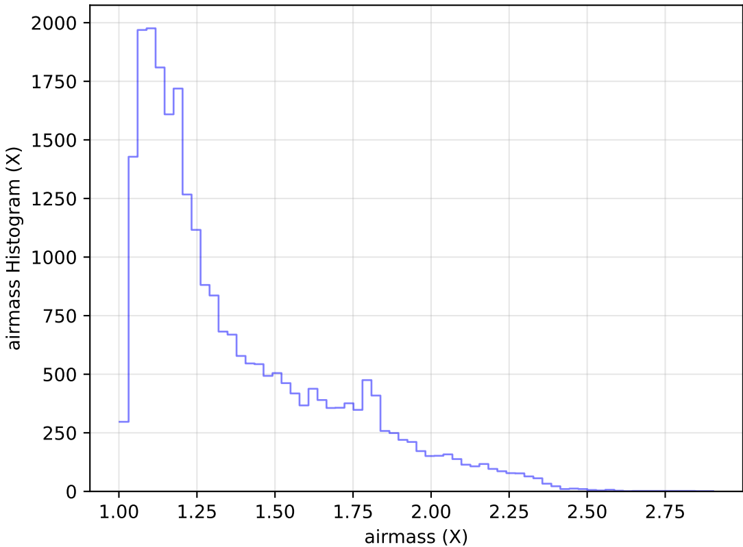
too_elab_r256_d3_ugrizy_v3.4_10yrs Yr 1 g band: airmass Histogram
