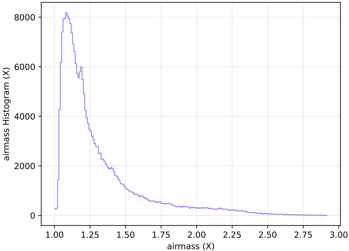
too_elab_r256_d3_ugrizy_v3.4_10yrs Yr 1 all bands: airmass Histogram
