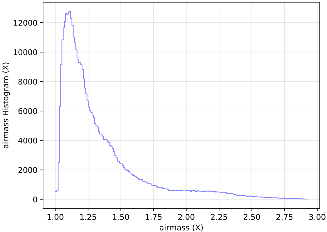
too_elab_r256_d3_ugrizy_v3.4_10yrs WFD z band: airmass Histogram
