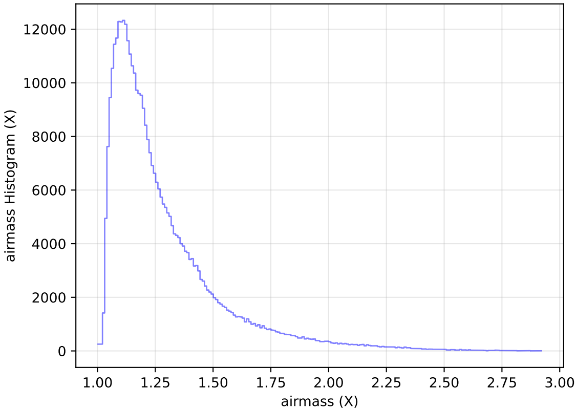
too_elab_r256_d3_ugrizy_v3.4_10yrs WFD y band: airmass Histogram
