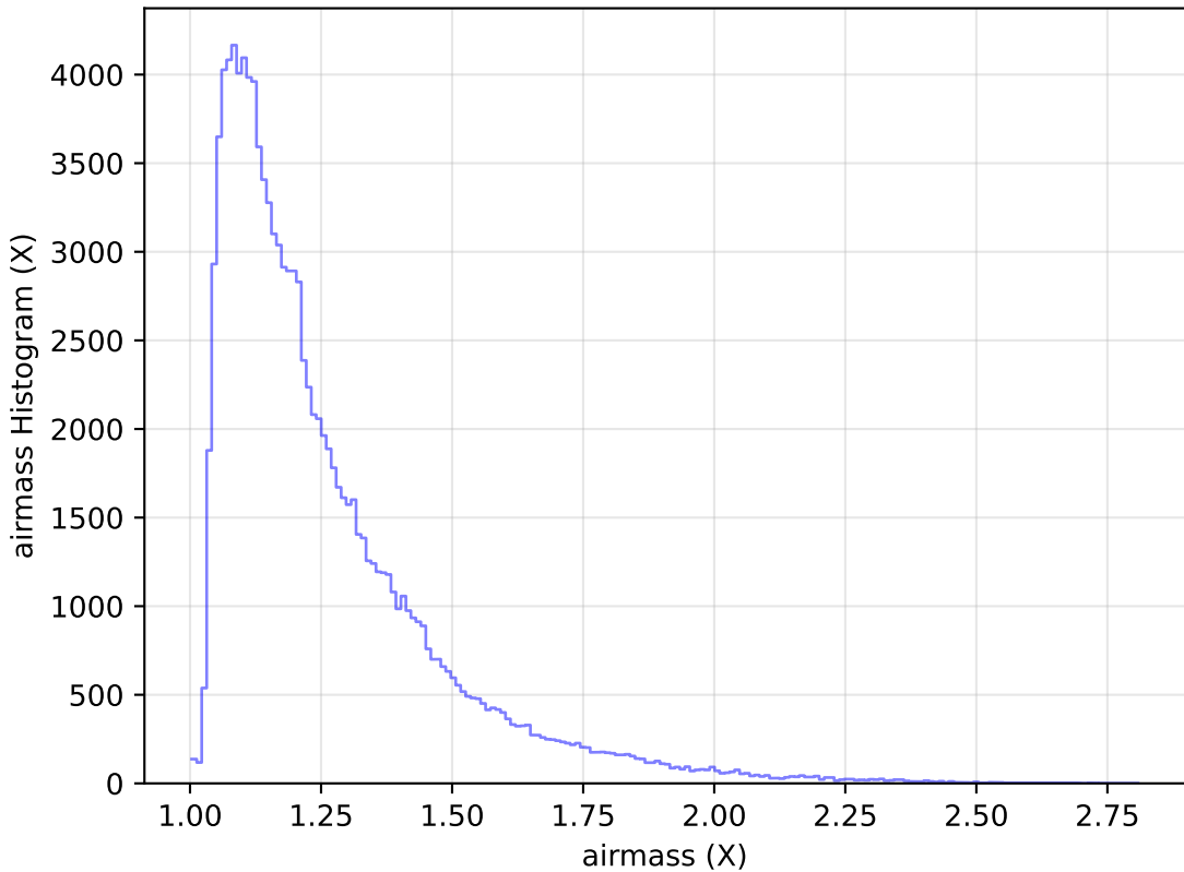
too_elab_r256_d3_ugrizy_v3.4_10yrs WFD u band: airmass Histogram
