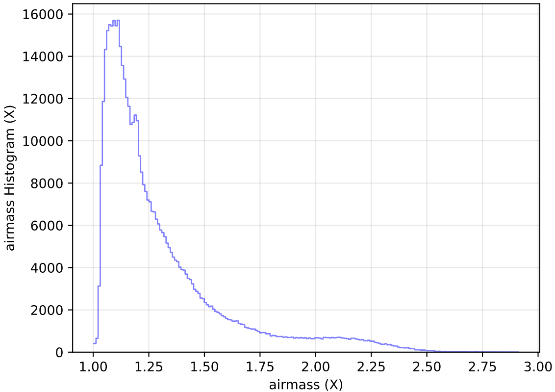
too_elab_r256_d3_ugrizy_v3.4_10yrs WFD r band: airmass Histogram
