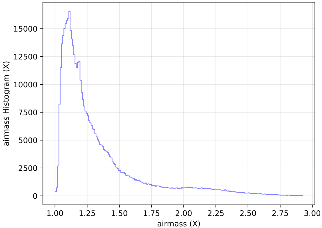
too_elab_r256_d3_ugrizy_v3.4_10yrs WFD i band: airmass Histogram
