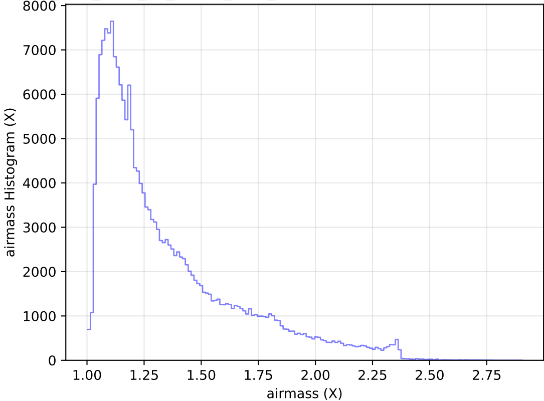
too_elab_r256_d3_ugrizy_v3.4_10yrs WFD g band: airmass Histogram
