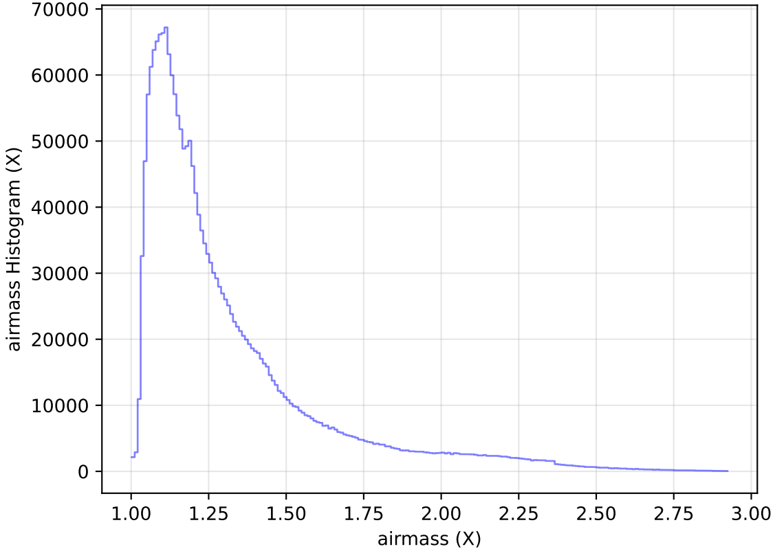
too_elab_r256_d3_ugrizy_v3.4_10yrs WFD all bands: airmass Histogram
