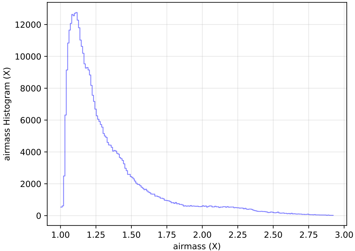
too_elab_r256_d3_ugrizy_v3.4_10yrs All sky z band: airmass Histogram
