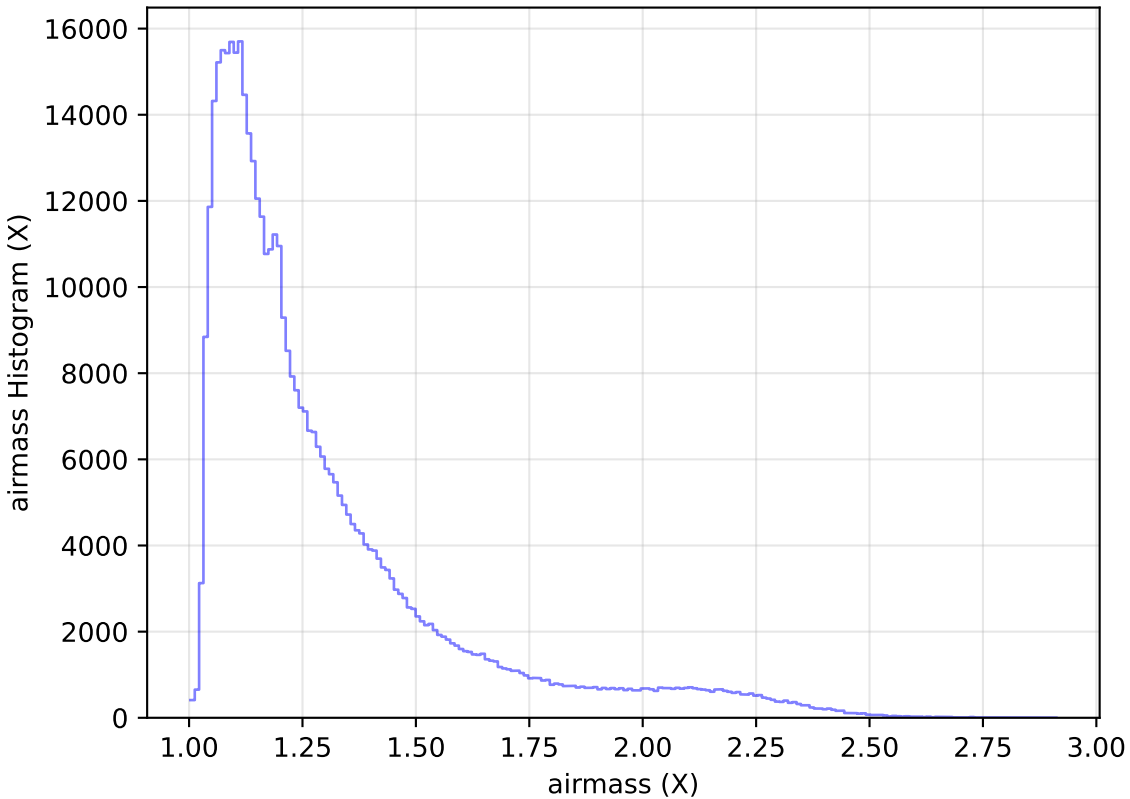
too_elab_r256_d3_ugrizy_v3.4_10yrs All sky r band: airmass Histogram
