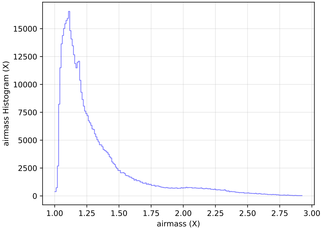
too_elab_r256_d3_ugrizy_v3.4_10yrs All sky i band: airmass Histogram
