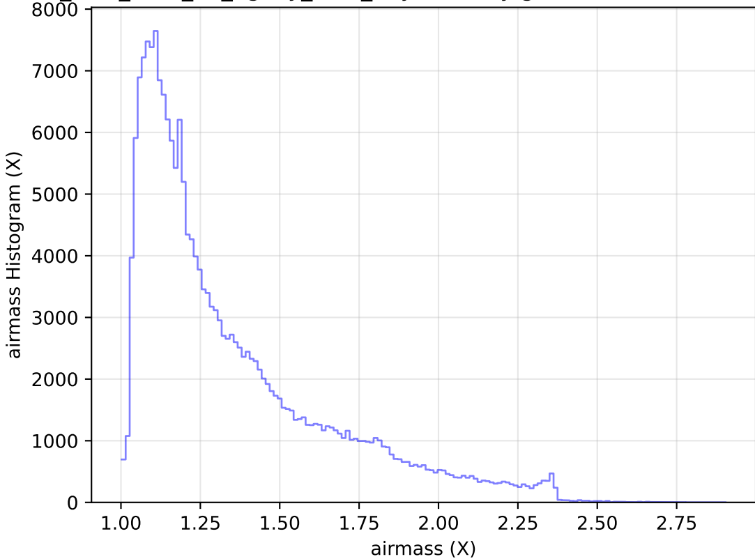
too_elab_r256_d3_ugrizy_v3.4_10yrs All sky g band: airmass Histogram
