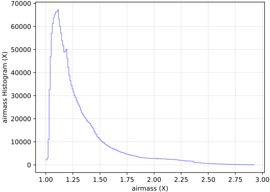
too_elab_r256_d3_ugrizy_v3.4_10yrs All sky all bands: airmass Histogram
