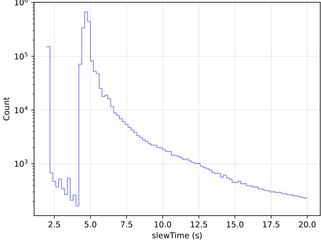
too_elab_r256_d3_ugrizy_v3.4_10yrs All visits: Zoom Slew Time Histogram
