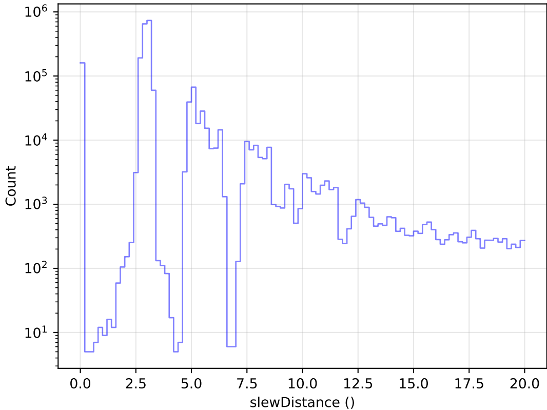
too_elab_r256_d3_ugrizy_v3.4_10yrs All visits: Zoom Slew Distance Histogram
