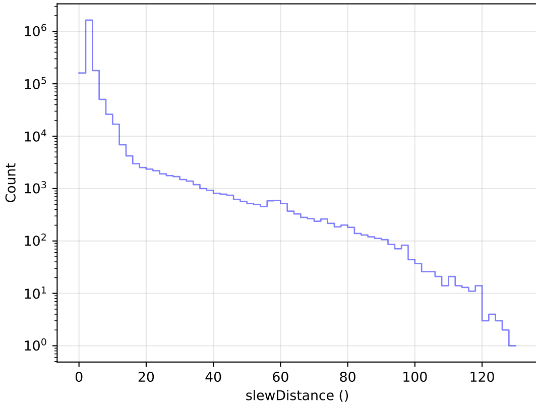
too_elab_r256_d3_ugrizy_v3.4_10yrs All visits: Slew Distance Histogram
