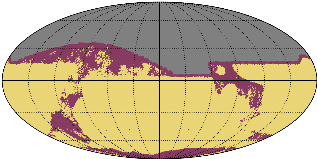
too_elab_r256_d3_ugrizy_v3.4_10yrs All sky: RapidRevisits
