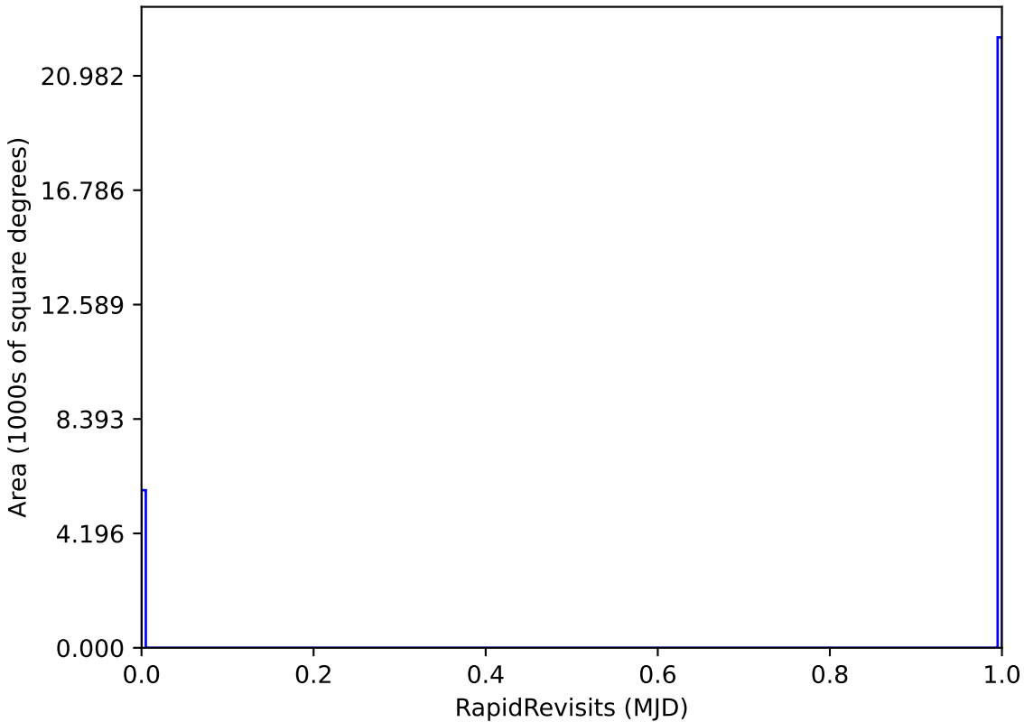
too_elab_r256_d3_ugrizy_v3.4_10yrs All sky: RapidRevisits
