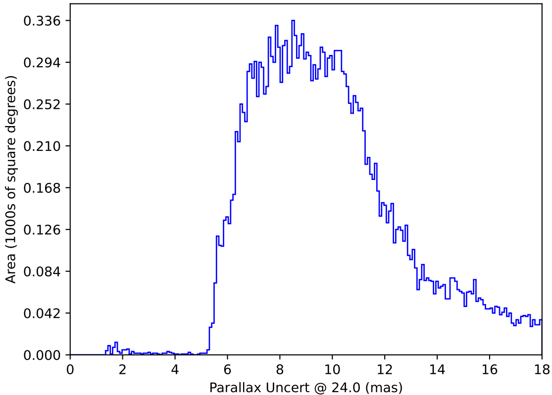
too_elab_r256_d3_ugrizy_v3.4_10yrs All sky: Parallax Uncert @ 24.0
