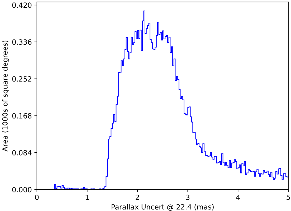
too_elab_r256_d3_ugrizy_v3.4_10yrs All sky: Parallax Uncert @ 22.4
