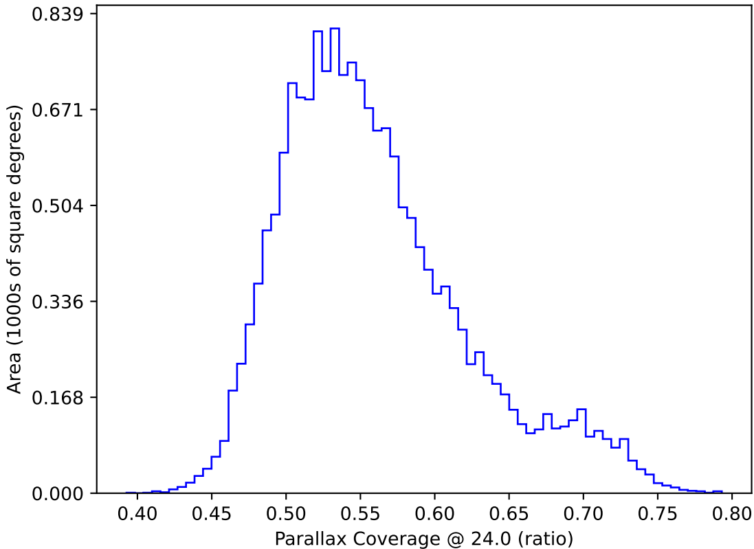
too_elab_r256_d3_ugrizy_v3.4_10yrs WFD: Parallax Coverage @ 24.0
