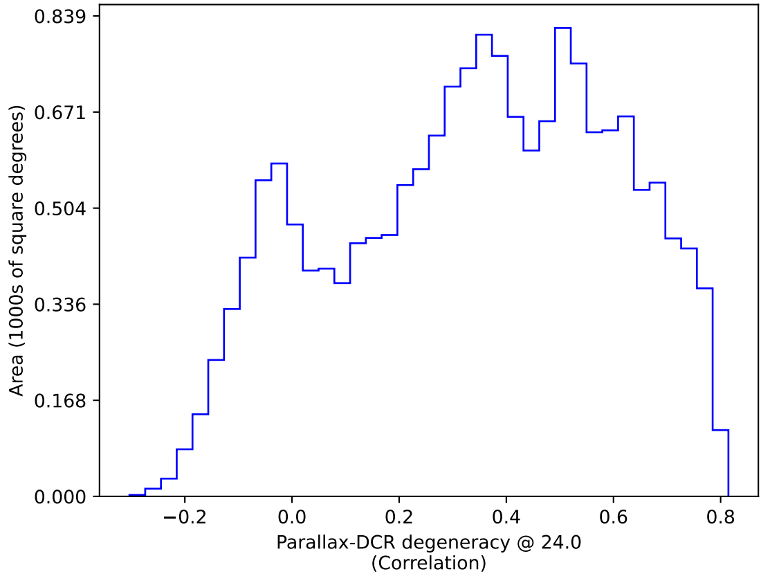
too_elab_r256_d3_ugrizy_v3.4_10yrs WFD: Parallax-DCR degeneracy @ 24.0
