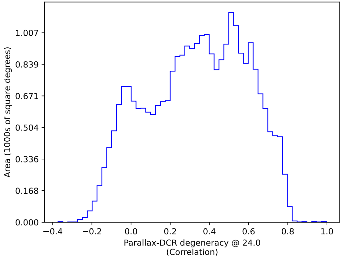
too_elab_r256_d3_ugrizy_v3.4_10yrs All sky: Parallax-DCR degeneracy @ 24.0
