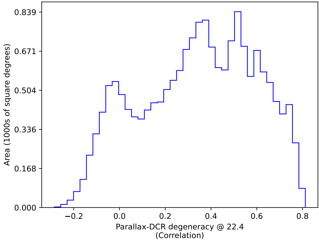
too_elab_r256_d3_ugrizy_v3.4_10yrs WFD: Parallax-DCR degeneracy @ 22.4
