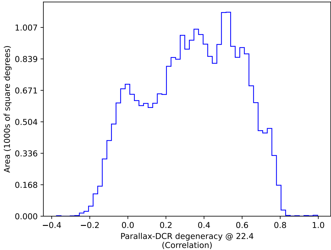
too_elab_r256_d3_ugrizy_v3.4_10yrs All sky: Parallax-DCR degeneracy @ 22.4
