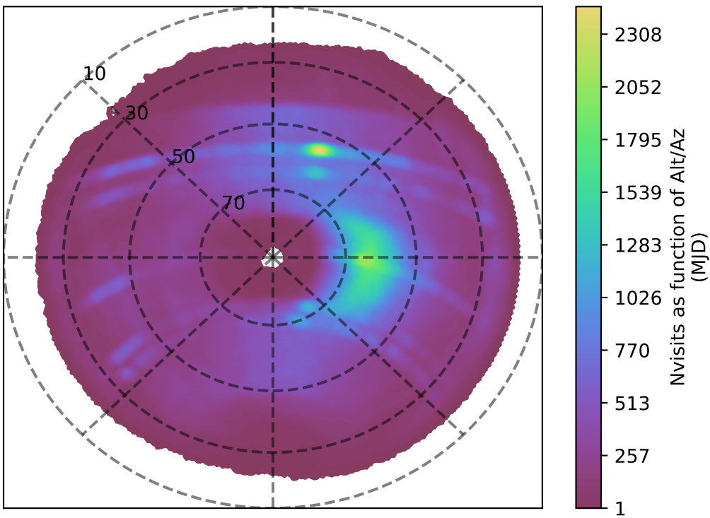
too_elab_r256_d3_ugrizy_v3.4_10yrs z band: Nvisits as function of Alt/Az
