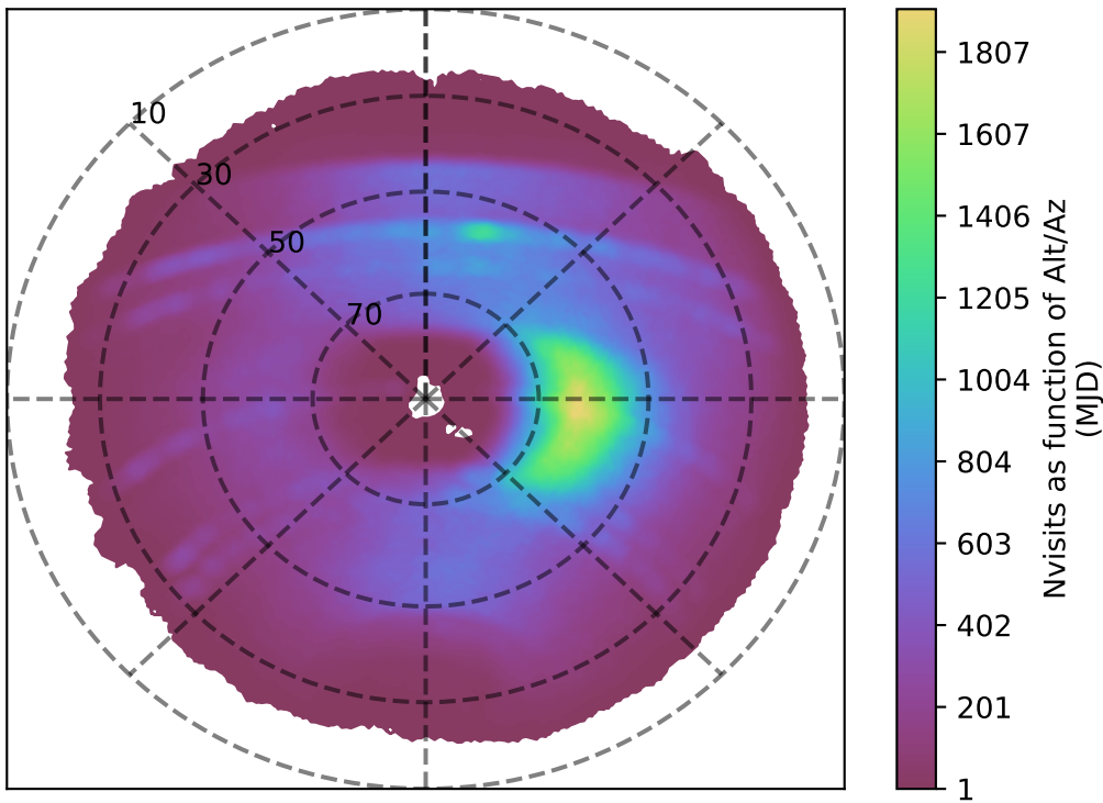
too_elab_r256_d3_ugrizy_v3.4_10yrs y band: Nvisits as function of Alt/Az
