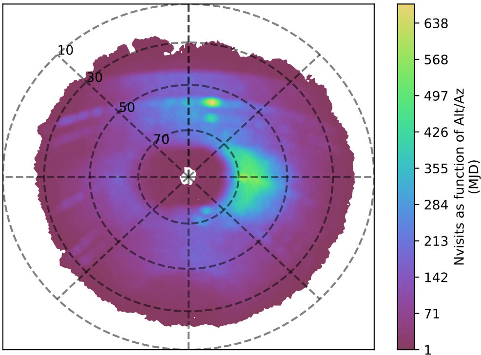
too_elab_r256_d3_ugrizy_v3.4_10yrs u band: Nvisits as function of Alt/Az
