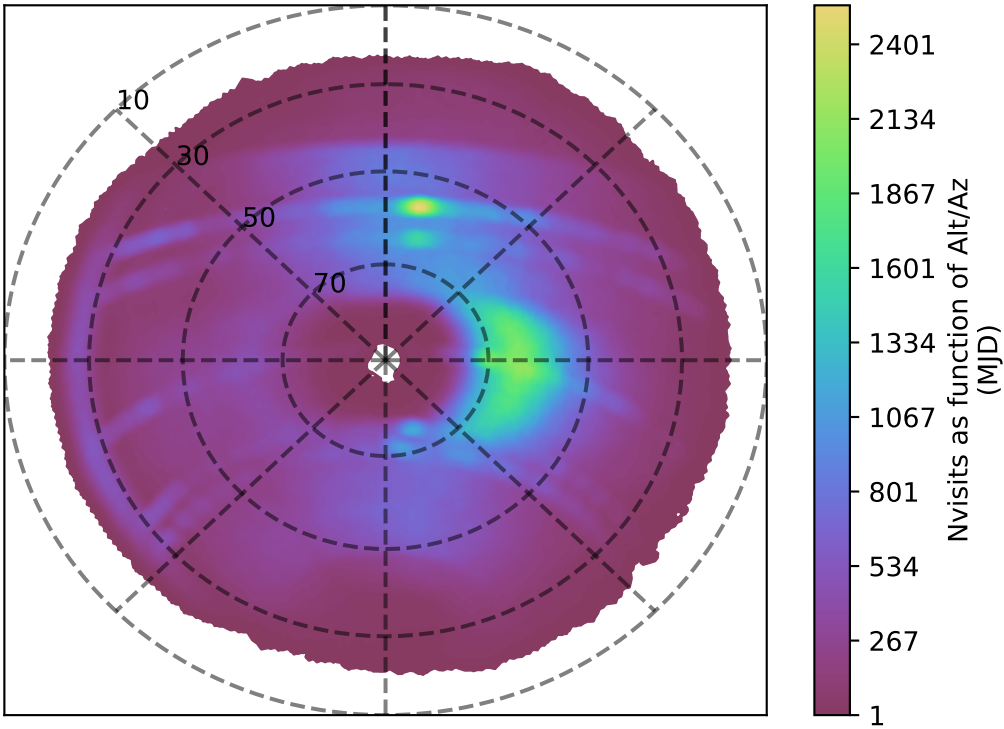
too_elab_r256_d3_ugrizy_v3.4_10yrs r band: Nvisits as function of Alt/Az
