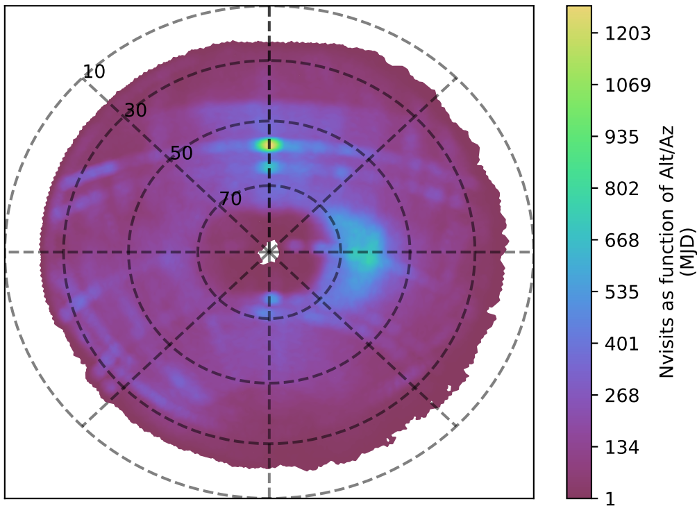
too_elab_r256_d3_ugrizy_v3.4_10yrs g band: Nvisits as function of Alt/Az
