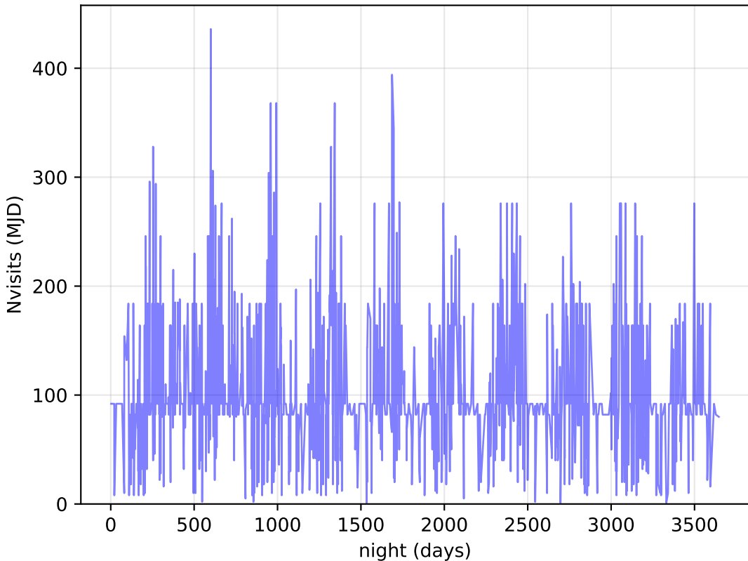
too_elab_r256_d3_ugrizy_v3.4_10yrs DDF: Nvisits
