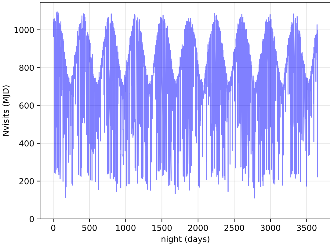
too_elab_r256_d3_ugrizy_v3.4_10yrs All visits: Nvisits
