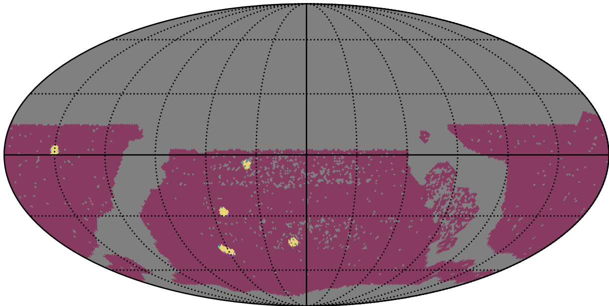
too_elab_r256_d3_ugrizy_v3.4_10yrs WFD: NumberOfQuickRevisits
