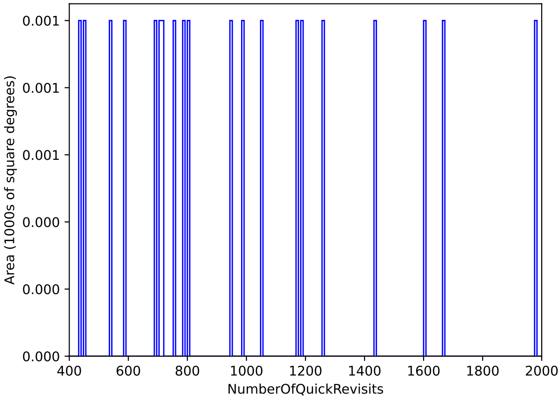
too_elab_r256_d3_ugrizy_v3.4_10yrs WFD: NumberOfQuickRevisits
