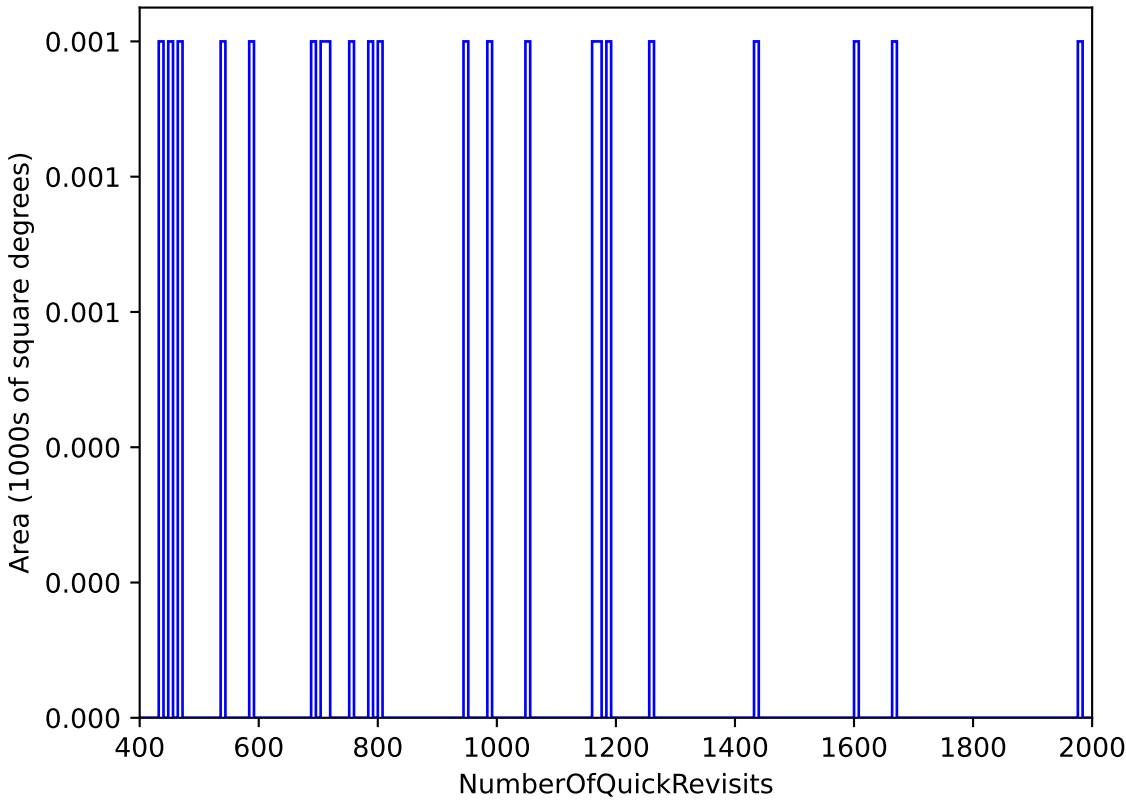
too_elab_r256_d3_ugrizy_v3.4_10yrs All sky: NumberOfQuickRevisits
