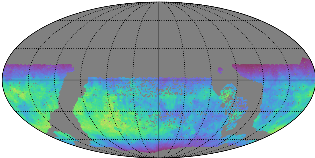
too_elab_r256_d3_ugrizy_v3.4_10yrs WFD z band: Normalized Teff
