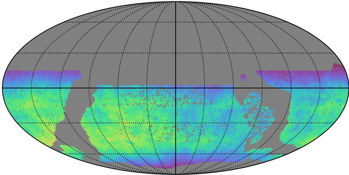
too_elab_r256_d3_ugrizy_v3.4_10yrs WFD y band: Normalized Teff
