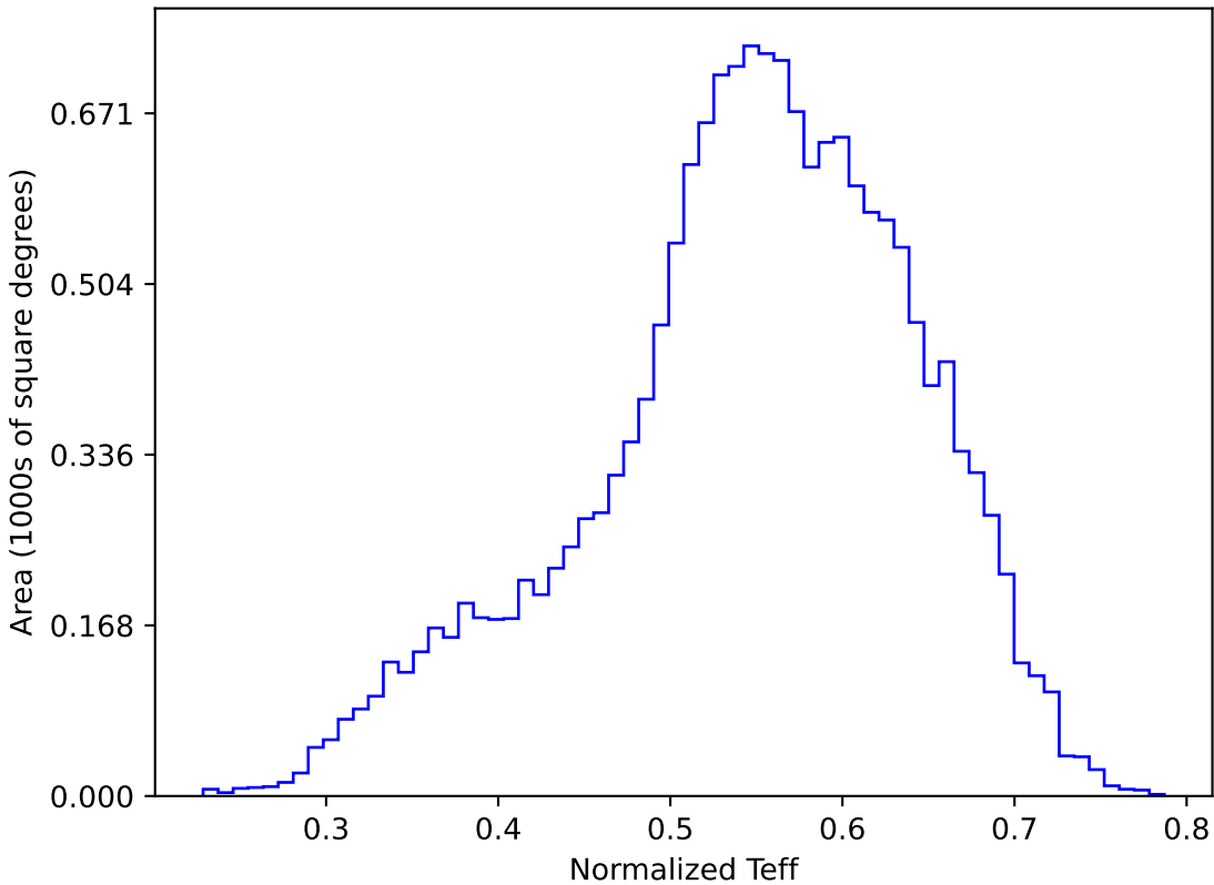
too_elab_r256_d3_ugrizy_v3.4_10yrs WFD y band: Normalized Teff
