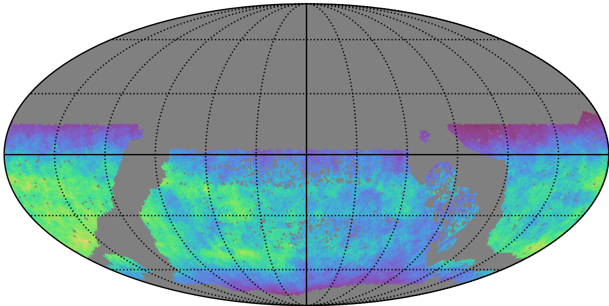
too_elab_r256_d3_ugrizy_v3.4_10yrs WFD u band: Normalized Teff
