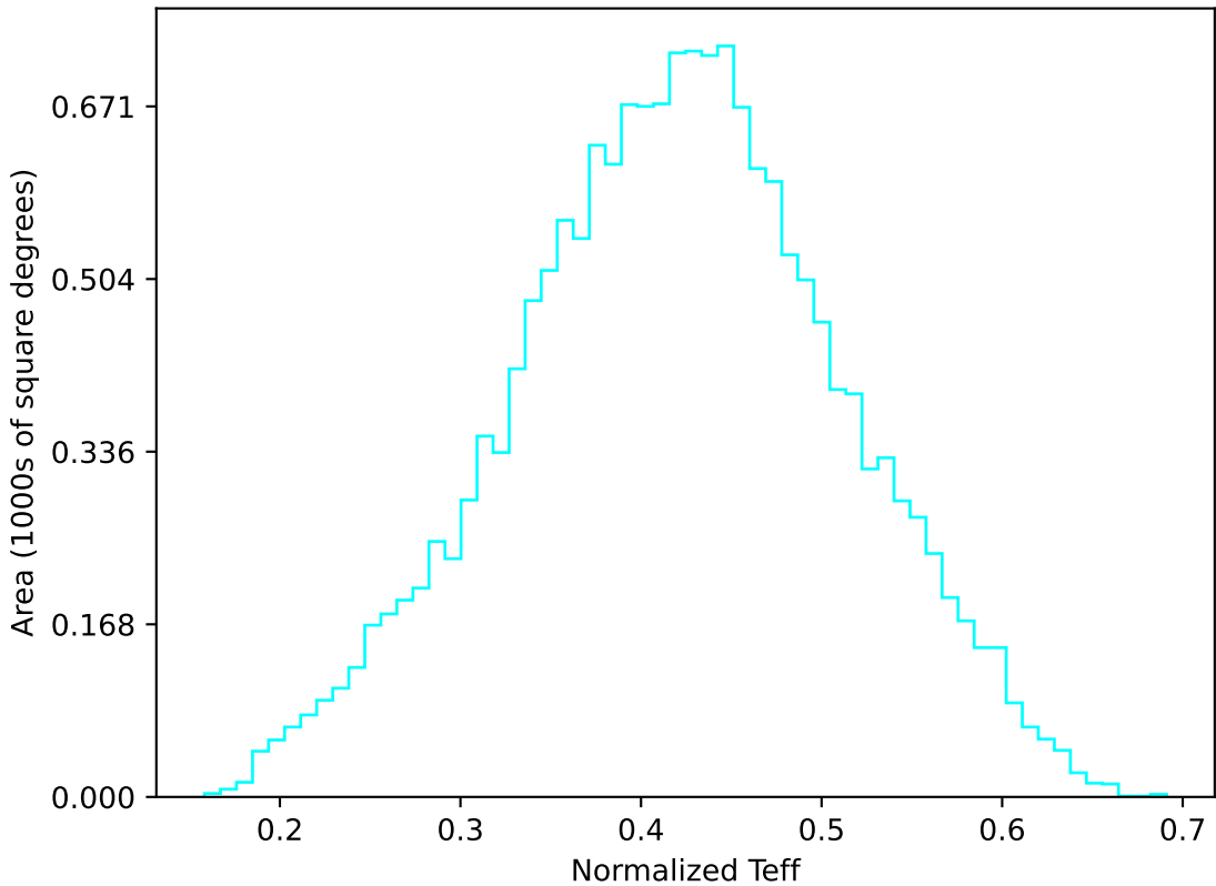
too_elab_r256_d3_ugrizy_v3.4_10yrs WFD u band: Normalized Teff
